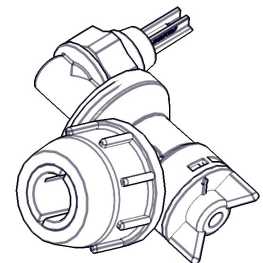
Valve "Closed"
